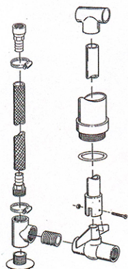
SOK10/SOK17 Shutoff and Drain Kit
